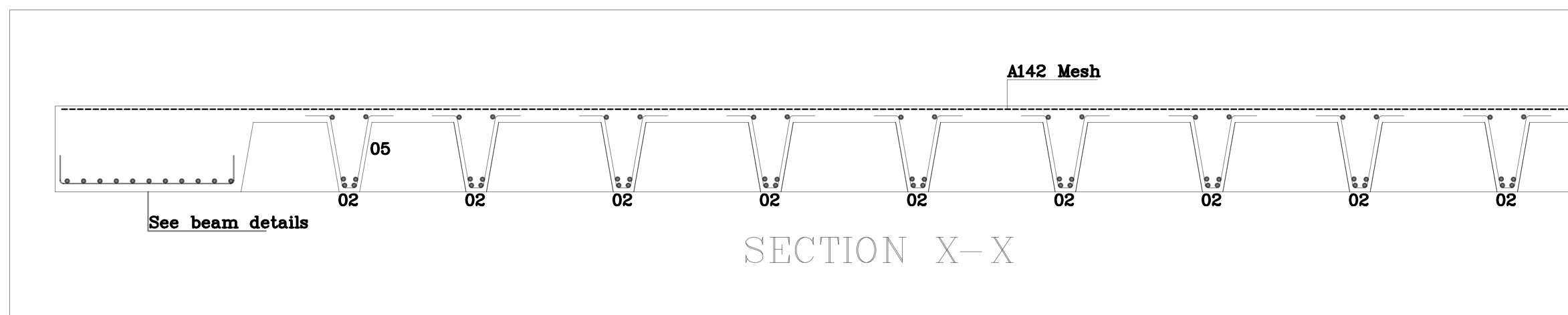
TYPICAL DETAILS OF END SPANS
