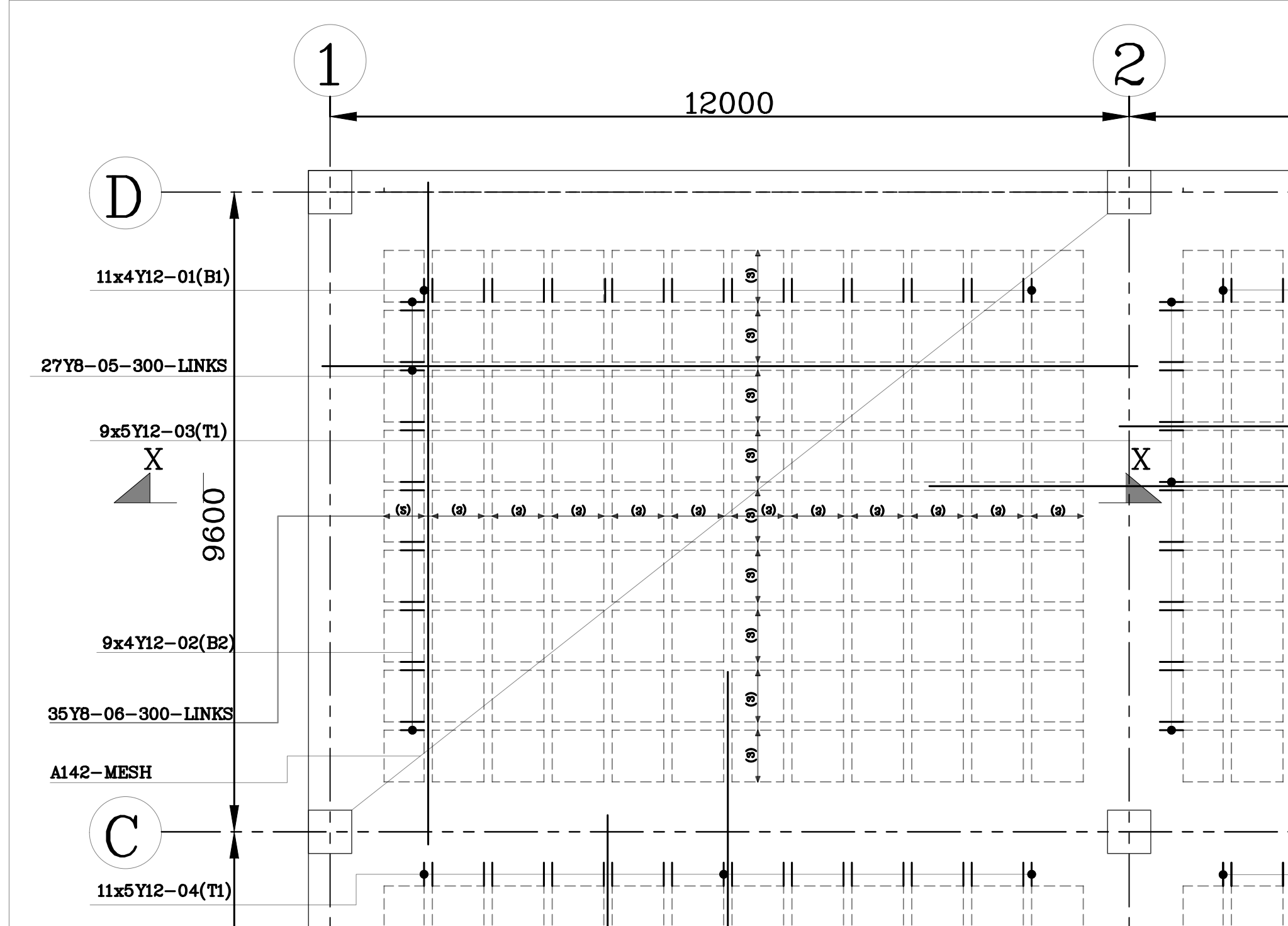
TYPICAL DETAILS OF END SPANS
